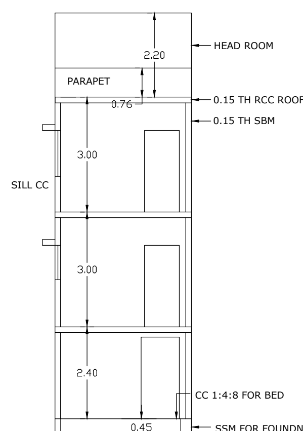
SECTION AA
